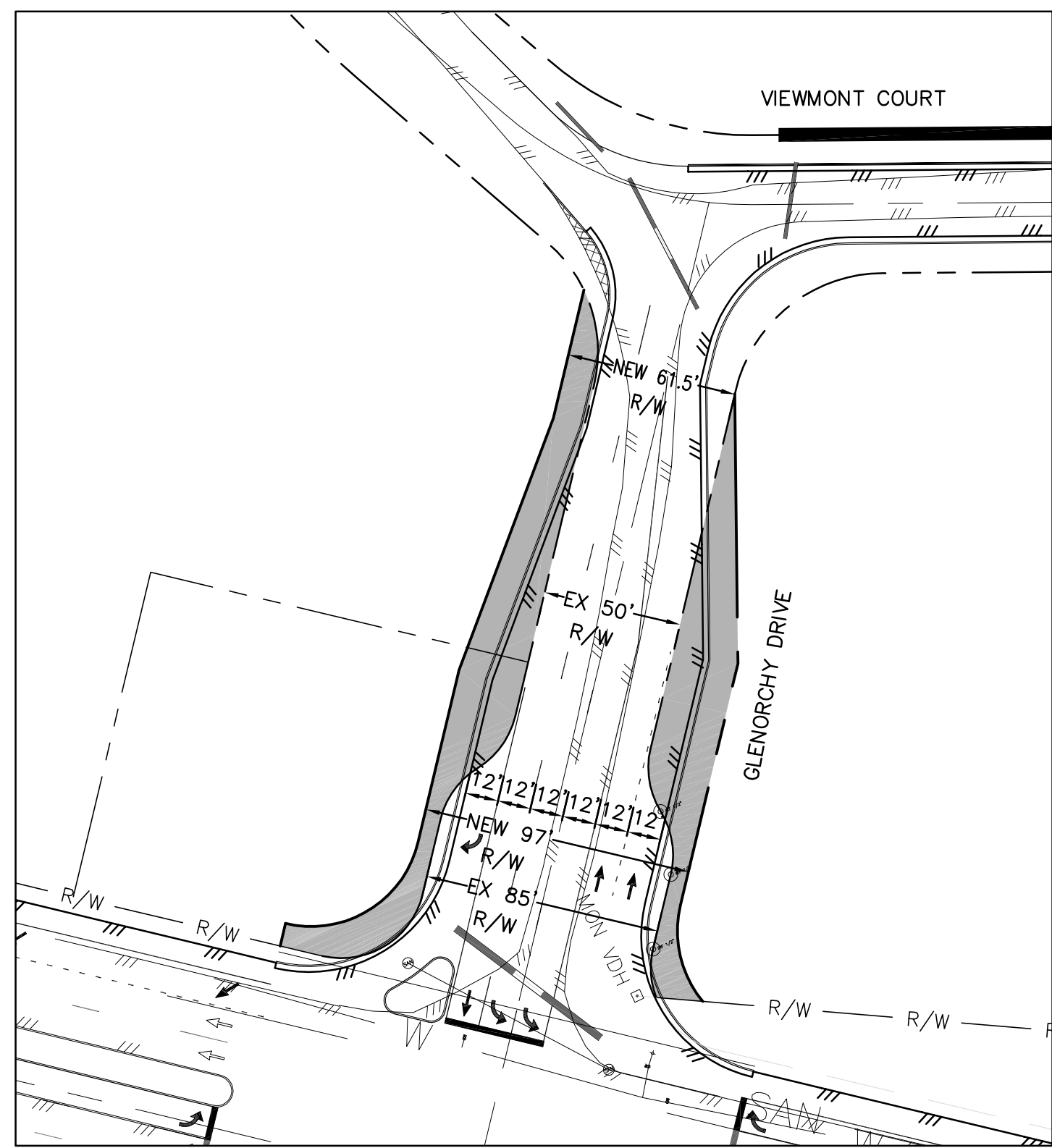
ENTRANCE DETAIL SCALE: 1"=50'
